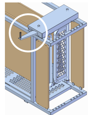
Strong handle for manual gate operation
